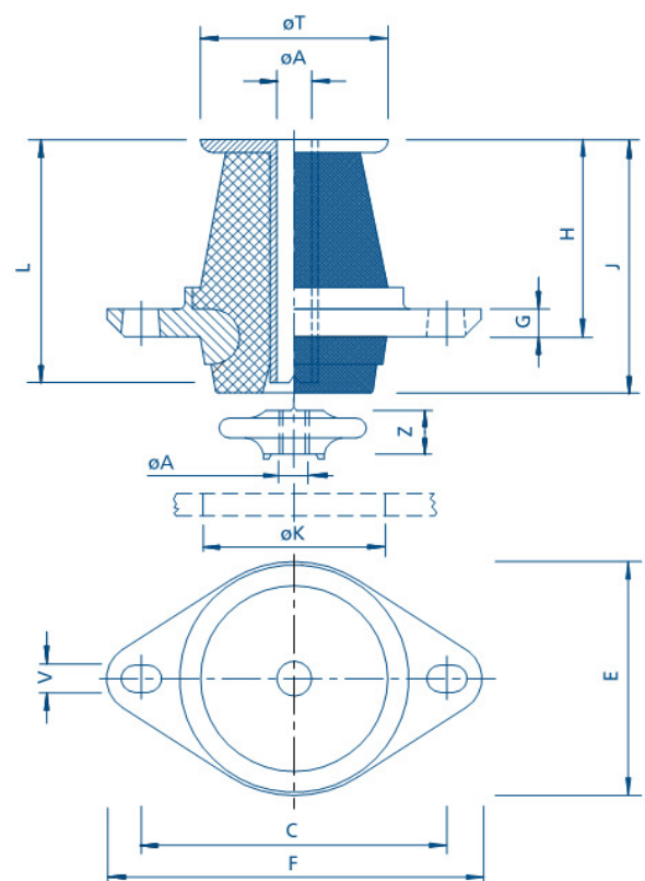
Figure 3: NF2000 Series
