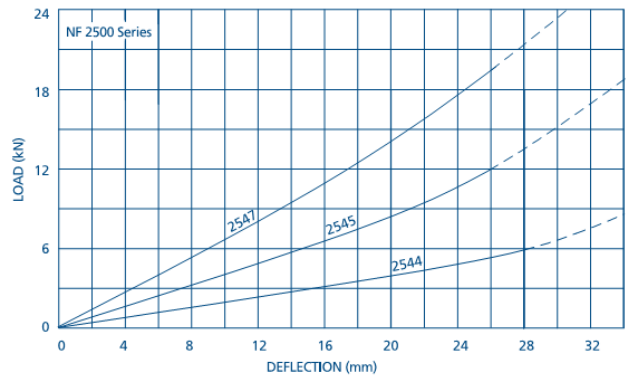
Figure 155: NF2500 Series Load Deflection
