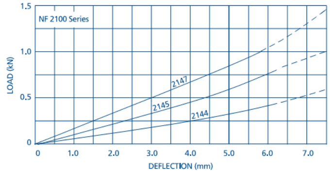
Figure 10: NF2100 Series Load Deflection
