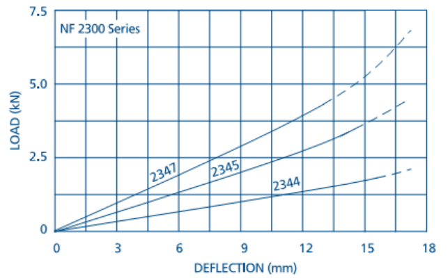
Figure 12: NF2300 Series Load Deflection
