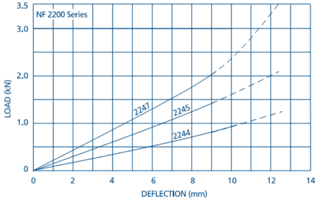
Figure 11: NF2200 Series Load Deflection
