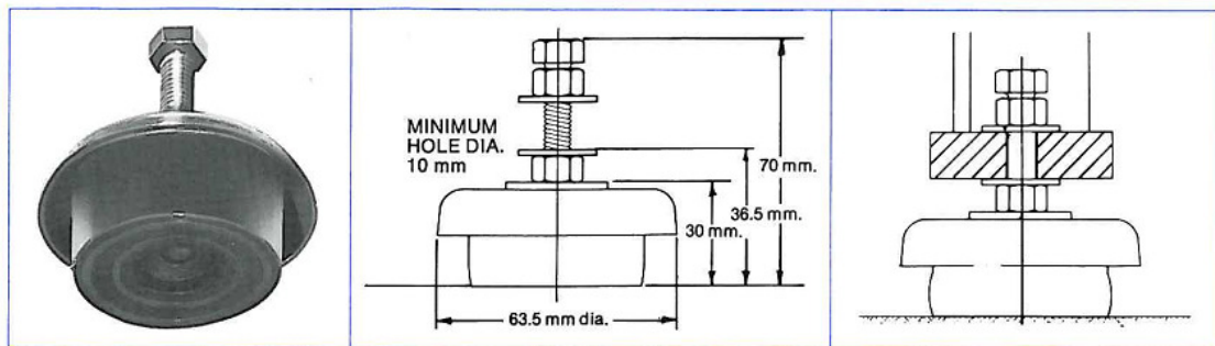
Figure 7: SLM100
