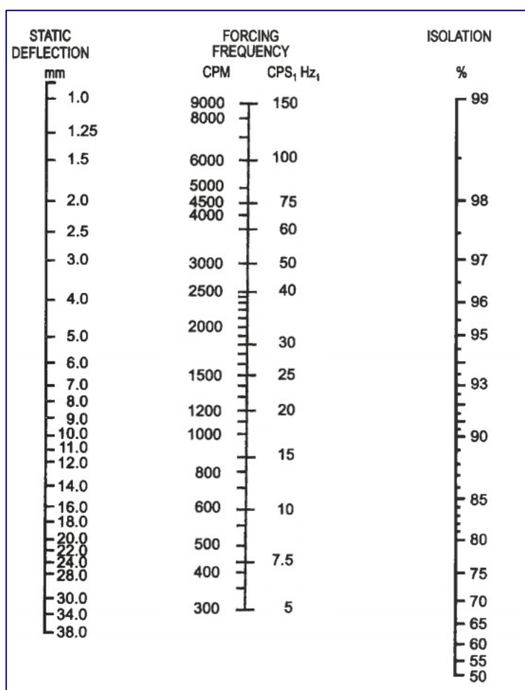
Figure 1: Isolation nomogram
