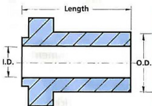
Universal Trunnion
