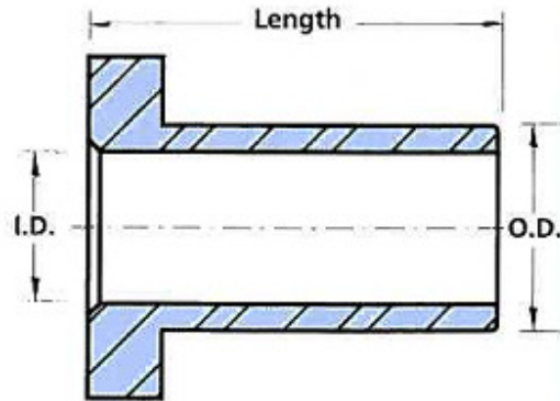
Hyflex Trunnion
