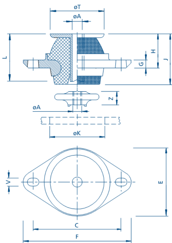
Figure 2: NF1000 Series
